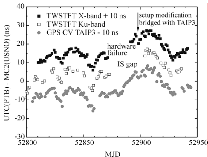
Figure 7. UTC (PTB) – MC2 (USNO) via three links (X-band, Ku-band, and TAI P3) in the vicinity of the so-called IS gap in August/September 2003. To achieve a better visualization, offsets of \pm 10 ns were applied to X-band and TAI P3, respectively.
