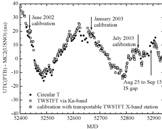
Figure 6. Circular T and Ku-band data of the timescale comparison UTC (PTB) – MC2 (USNO). Calibration dates and results (diamonds) are shown as well as the so-called INTELSAT (IS) gap.
